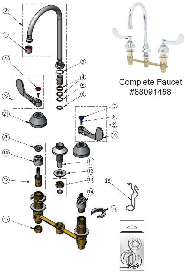
99316279 Installation Repair Kit Includes #12, (2)#16, & #15
